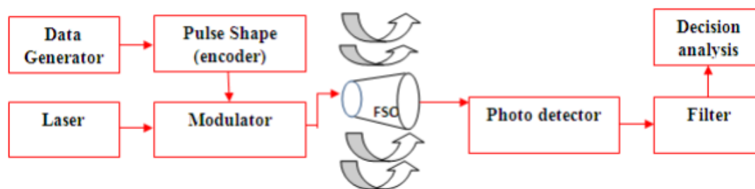
Fig. 4.1 Block diagram of FSO Communication System
